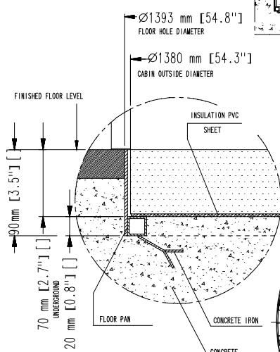
DETAIL "A" FLOOR PAN DETAIL
