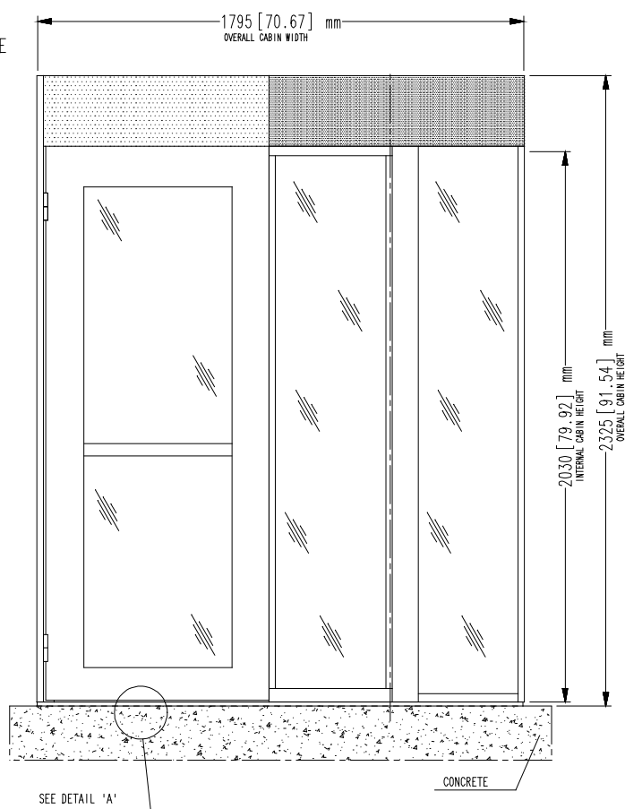
FRONT VIEW EXTERNAL SIDE
