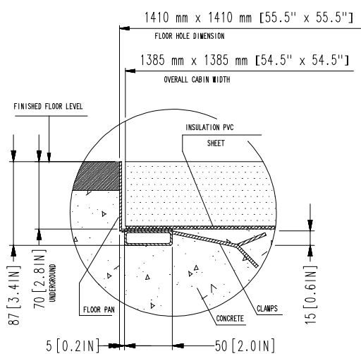
FLOOR PAN DETAIL
